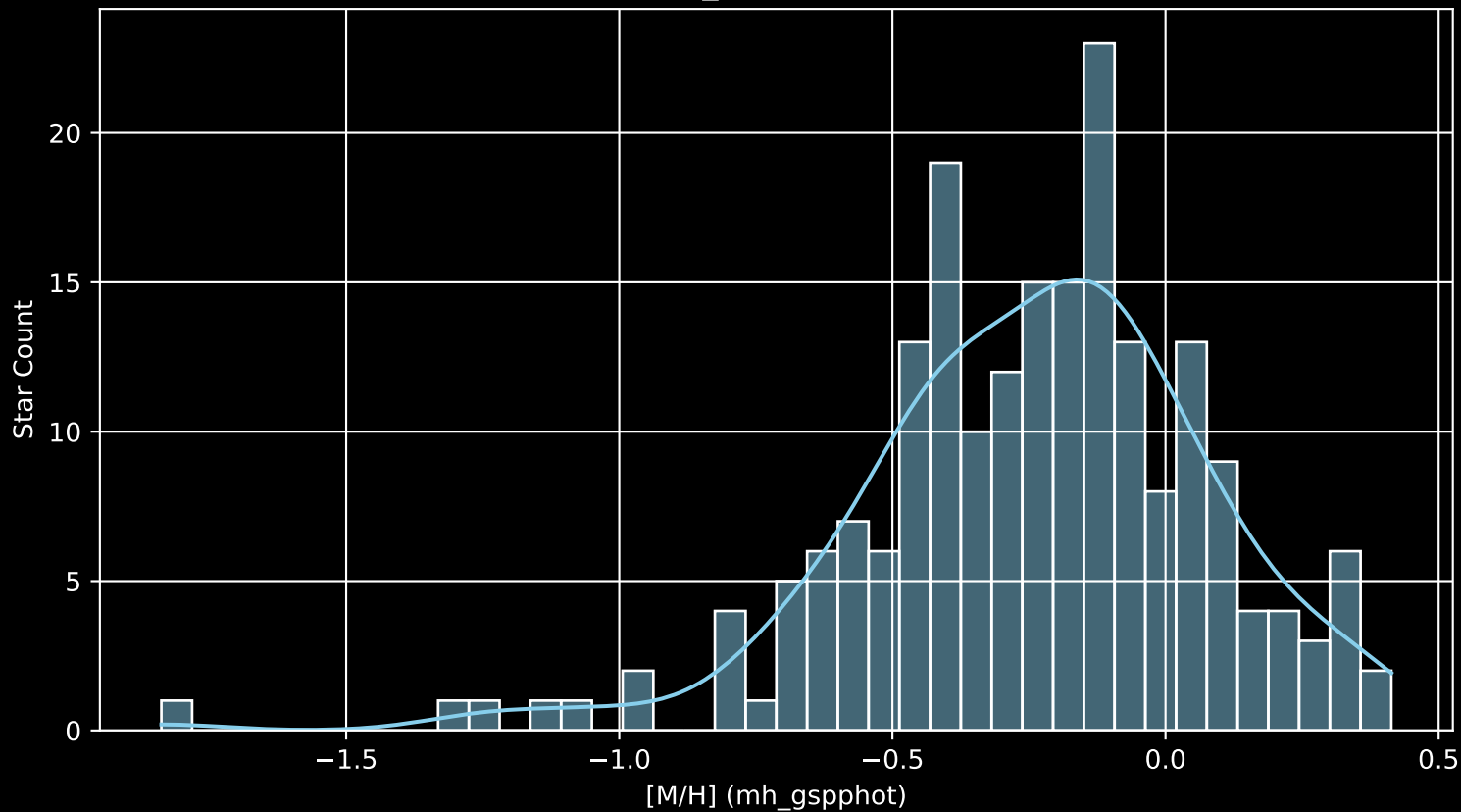
APOGEE DR17 Field: [K2_C12_069-65_btx [M/H] (mh_gspphot) (n= 205)
