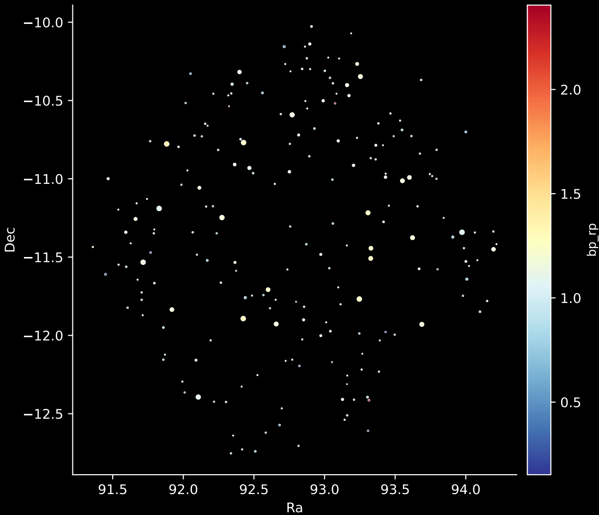
APOGEE DR17 Field: [K2_C12_069-65_btx] Stars: 206
