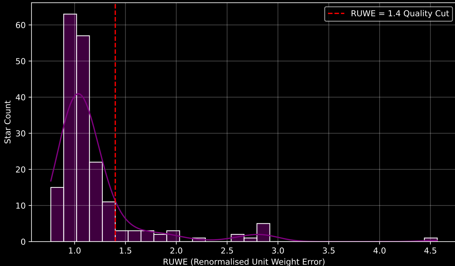
GAPOGEE DR17 Field [K2_C12_069-65_btx] RUWE Distribution (n= 192)
