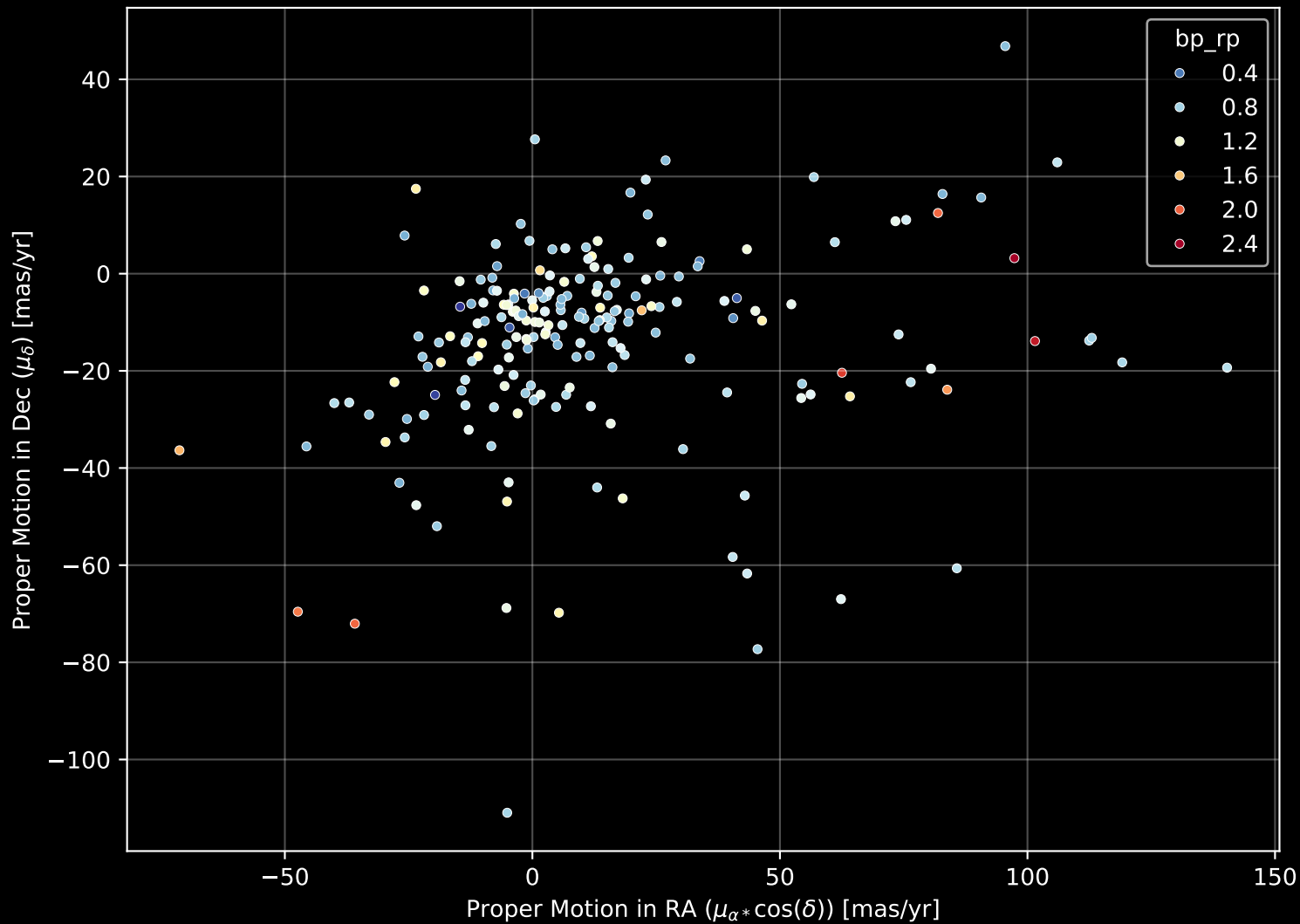
APOGEE DR17 Field: [K2_C12_069-65_btx] Proper Motion Diagram (n= 206)
