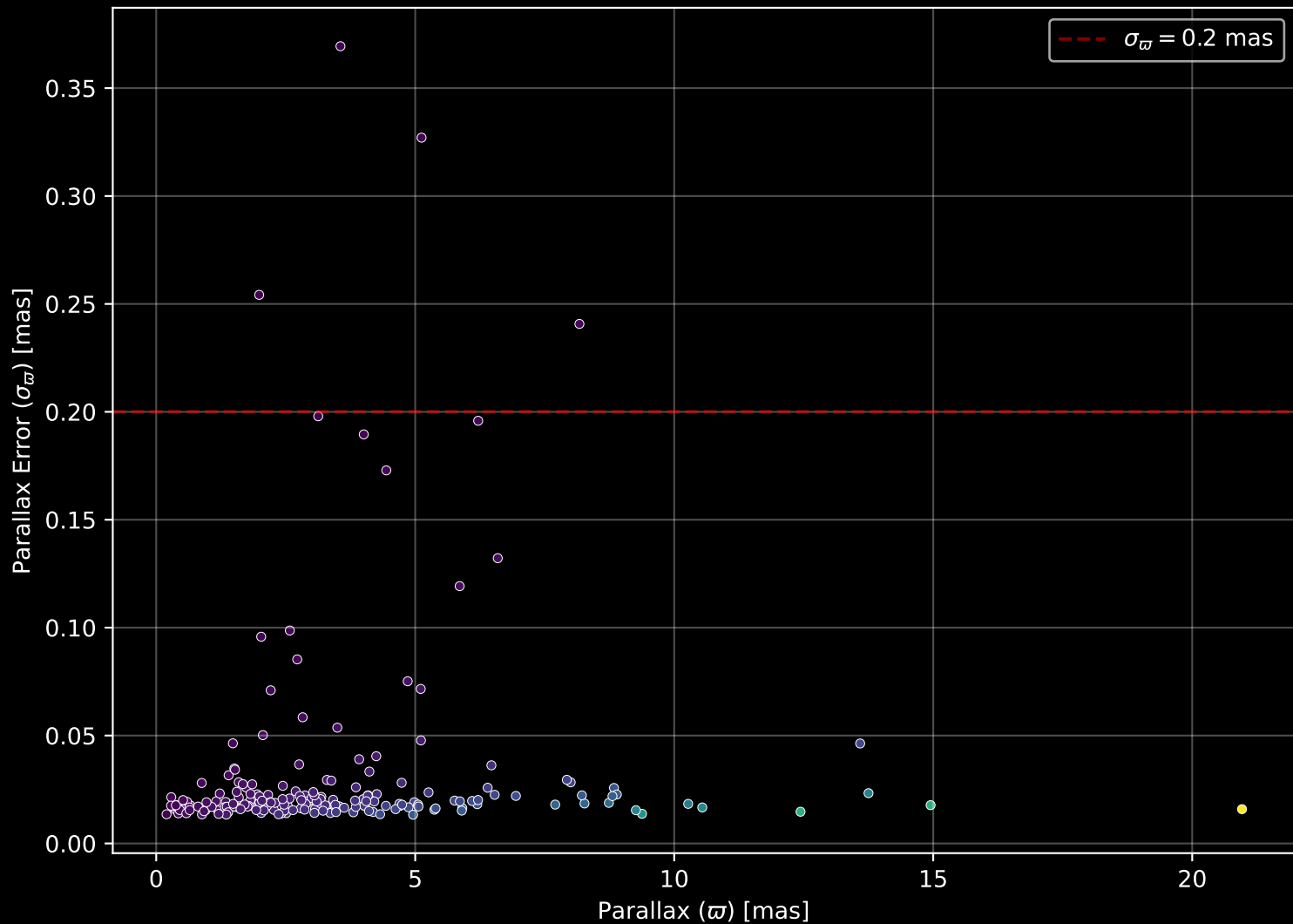
APOGEE DR17 Field: [K2_C12_069-65_btx] Parallax Quality (n= 206)
