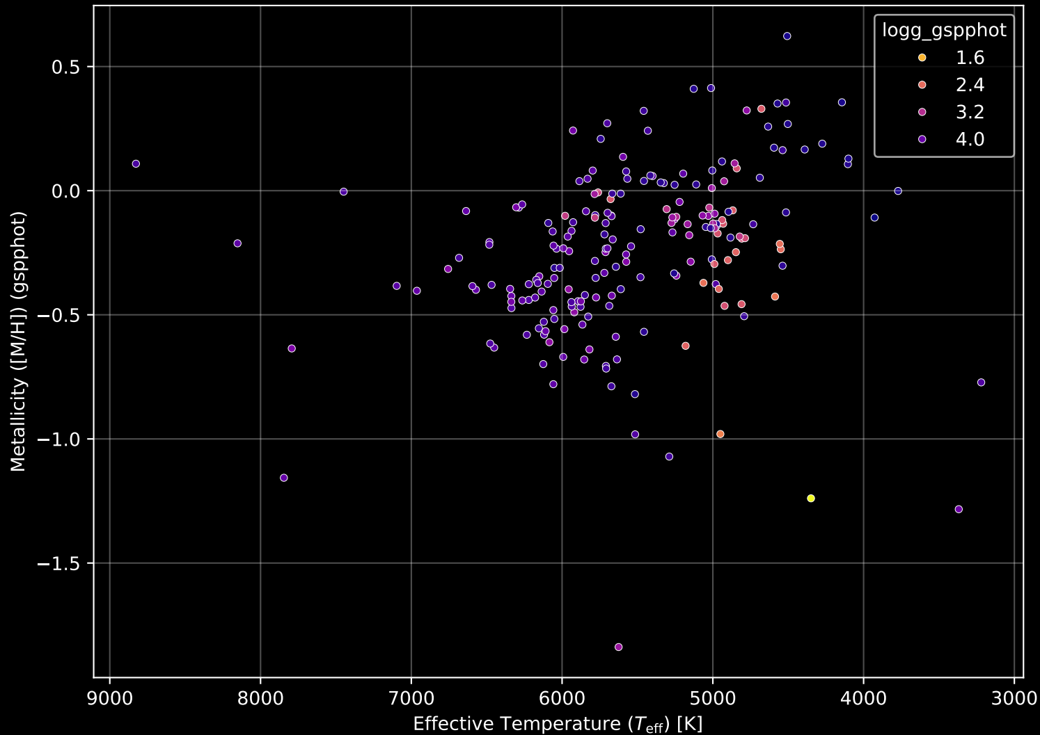
APOGEE DR17 Field: [K2_C12_069-65_btx] Stellar Population Parameters (n= 206)
