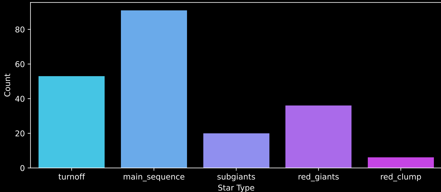
APOGEE DR17 Field: [K2_C12_069-65_btx] Count plot of Star Type
