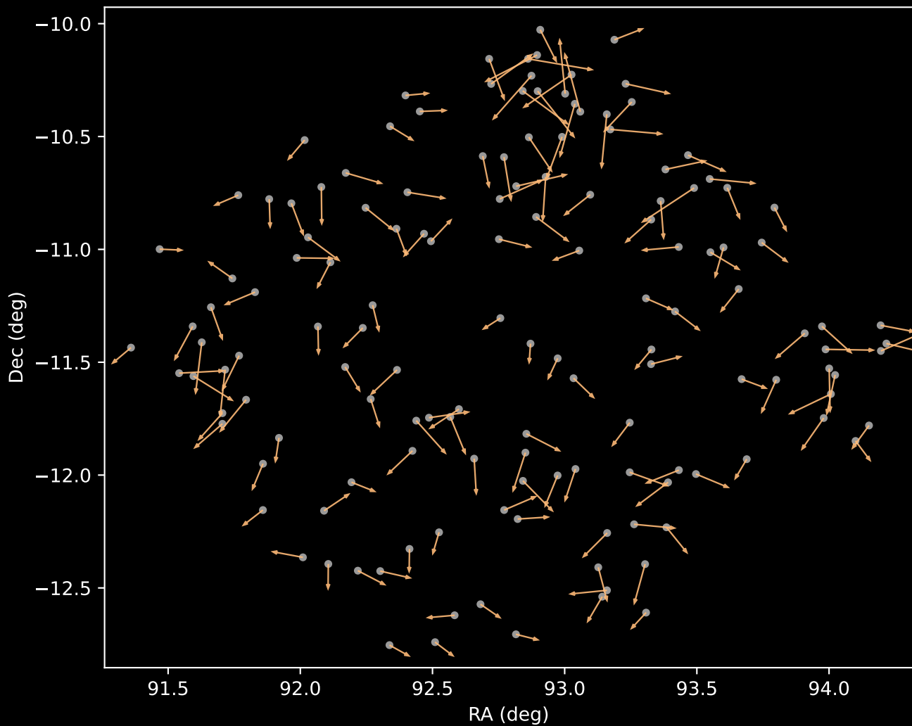
APOGEE DR17 Cluster 3 Proper Motion Vectors (n=143)
